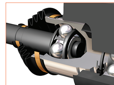
3 CV JOINT
