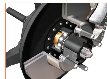
5 FRONT HUB
