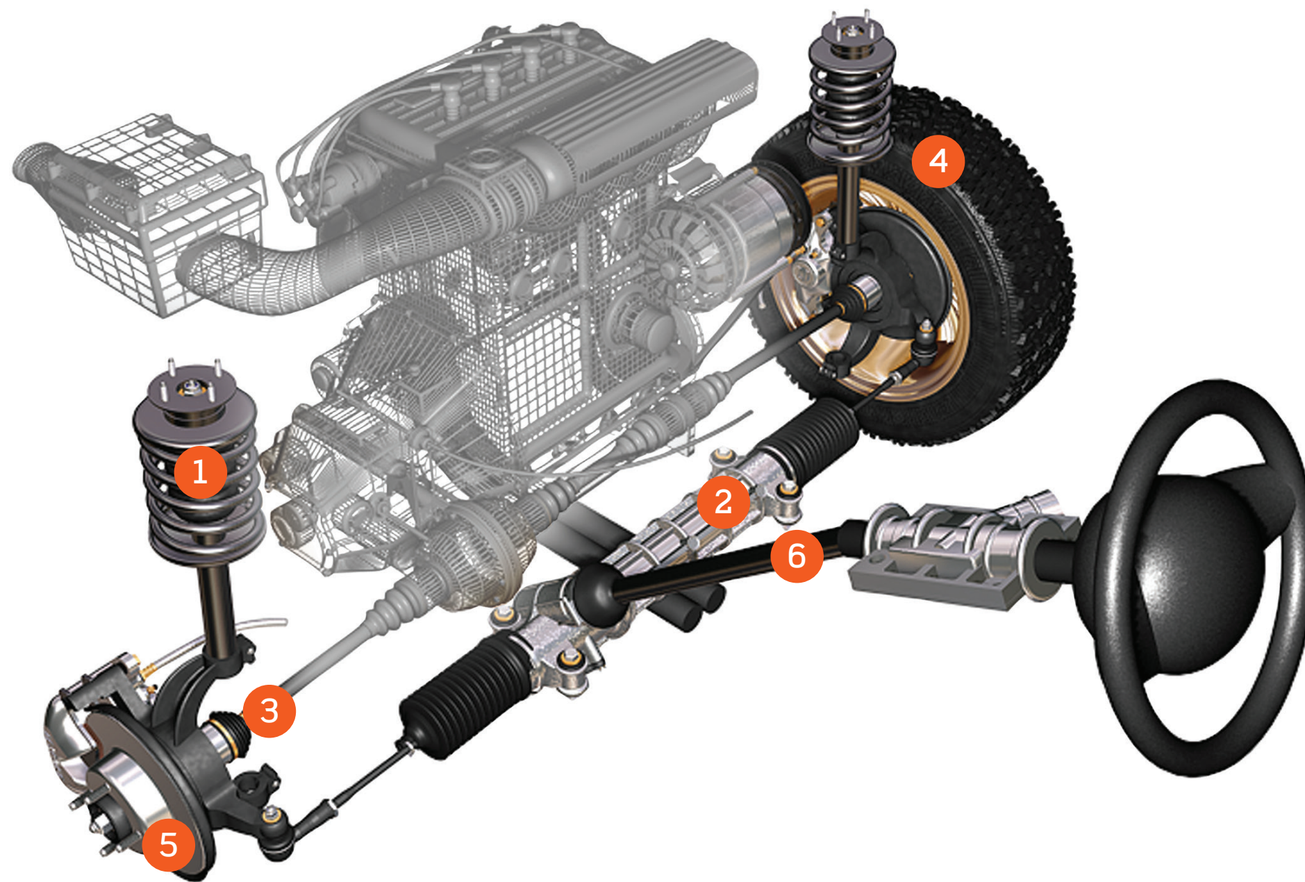
1 SUSPENSION
