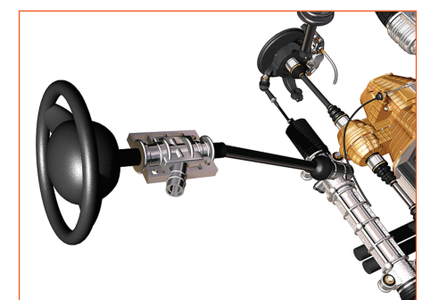
6 STEERING COLUMN
