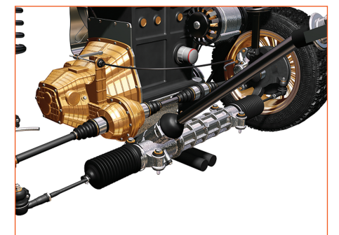
2 STEERING RACK
