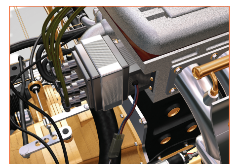
6 IGNITION COILS
